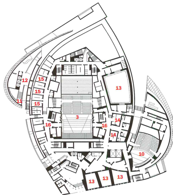
STAGE LEVEL
