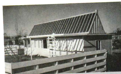
Another view of the house with "sun-measuring" gadgets called pyrheliometers evident on the eaves and peak (right) of the roof. They measure the intensity of solar radiation outside a collector tilted at the 57 degree angle or oriented vertically.
