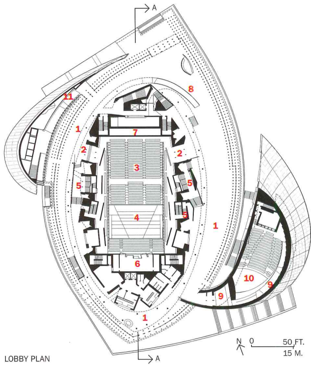
LOBBY PLAN
