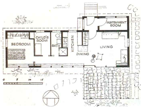
Floor plan, 1949 MIT solar test house, with an equipment room for the solar heating system about as large as the child's bedroom.
