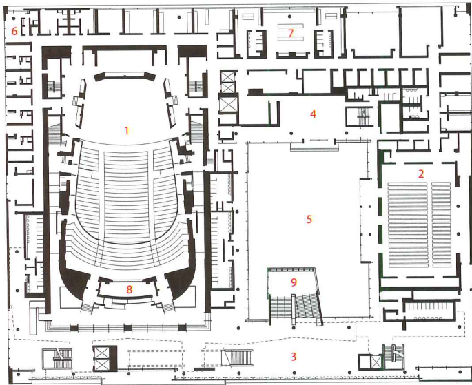
ORCHESTRA LEVEL
