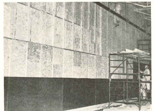
Building is group of huge deep-freeze rooms surrounded by corridors and loading docks. A nice problem was to keep floors from heaving due to frost formation in sub-soil. A grid of vitrified tile, acting as air ducts, was installed under heavily insulated concrete floor. Thermocouples show when temperature drops to freezing, when heated air is introduced into the ducts
