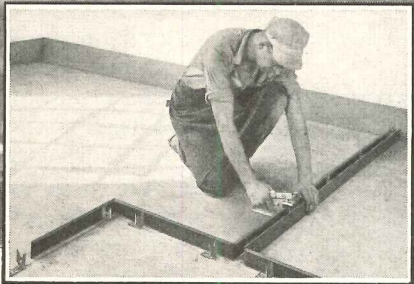
Wheeling Metal Base firmly locks into position on both sides of Floor Clips. Ceiling Runner goes up easily using stub nails or rawl drives.
