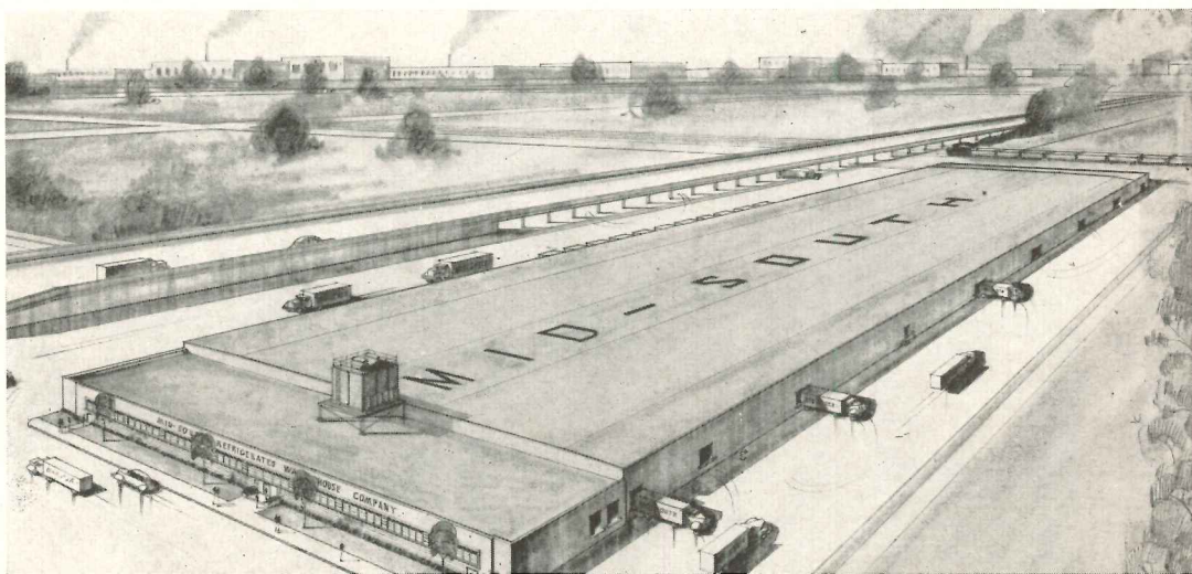
Building is group of huge deep-freeze rooms surrounded by corridors and loading docks. A nice problem was to keep floors from heaving due to frost formation in sub-soil. A grid of vitrified tile, acting as air ducts, was installed under heavily insulated concrete floor. Thermocouples show when temperature drops to freezing, when heated air is introduced into the ducts
