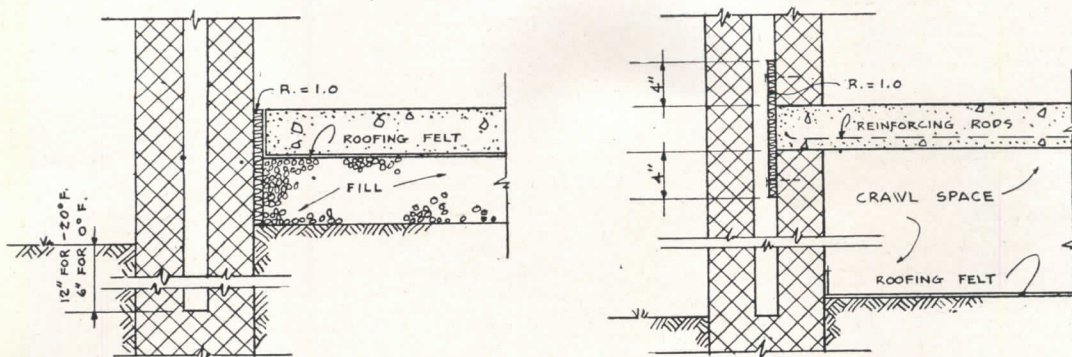
CAVITY WALLS
