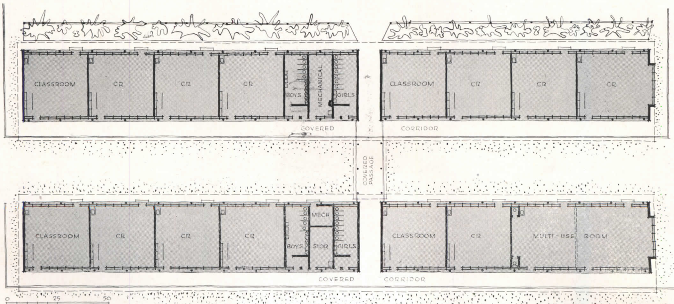
Plan provides for an eight-grade program, using duplicate rooms. Through-passage does not interrupt roofs (see section, page 85)
