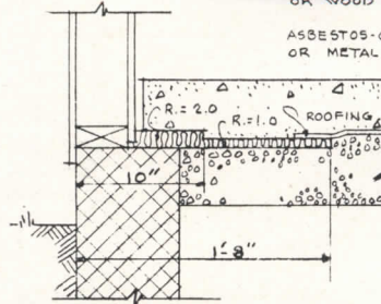
CONCRETE SLAB ON GROUND
