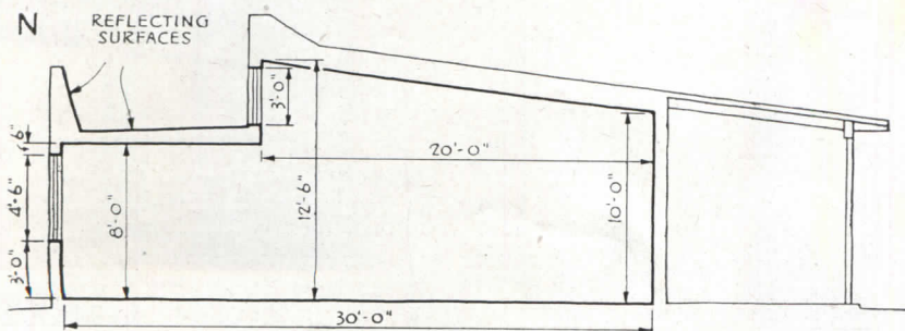
B. Parapet as a reflector is very effective, judged by fact that when it was blacked, readings at interior wall were reduced from 50 to 28 fc. On a clear March day at 2 p.m., intensity was virtually level at 50 fc., with a rise to 53 fc. at approximate center line. In December, at 1:45 p.m. with rain, the curve was: 8 ft. from window, 26 fc.; 18 ft., 45 fc.; 28 ft., 22 fc. Paso Robles School, Frank Wynkoop & Associates
