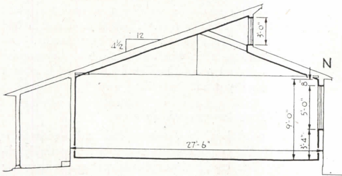
A. Light thrown well back into the room from high up, though maximum possible window area is only 29% of floor area. Readings not yet available. Montalvo Migratory School, California, R. S. Raymond
