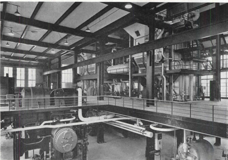
Interior of the Burroughs power plant. It was one of the first plants to break away from the common practice of putting a partition between boiler and generator rooms. Coal dust is not allowed to escape
