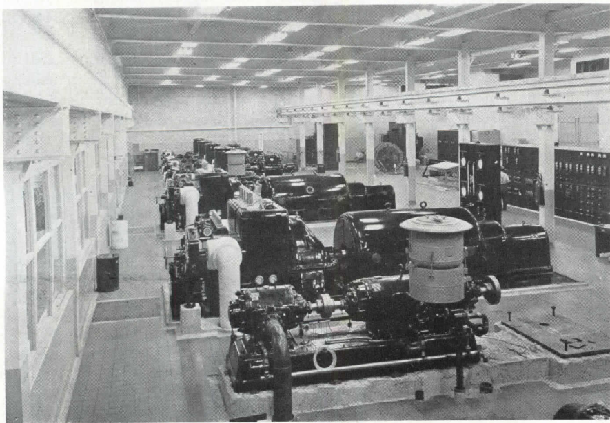
General view of air compressors and turbo-generators in the Willow Run power house. Note the overhead cranes, which are always included in generator or air compressor rooms to facilitate repairs
