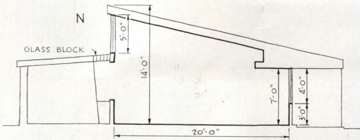
G. Glass block, used as skylight in corridor ceiling, admit light down through the showcase underneath and diminish the effect of brightness contrast. Louvers or additional block would probably be needed at clerestory window to cut down sky glare. View windows to south require no control devices, being well shaded. Proposal by Richard J. Neutra in the March, 1944, issue of the ARCHITECTURAL RECORD
