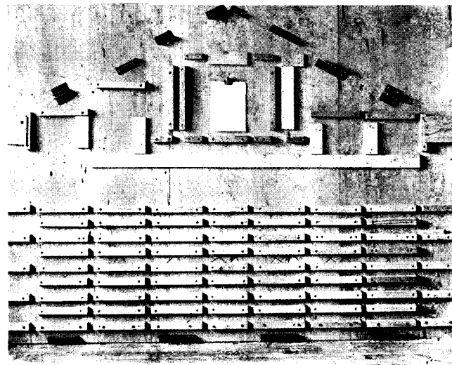
One jig table (American Houses) serves for many panel types
