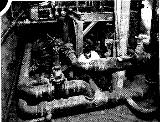
Steam heat for the entire Terrace Village is supplied through 10" seamless mains while 6" laterals serve steam to various block sections. 4" pipe is used for the return.
