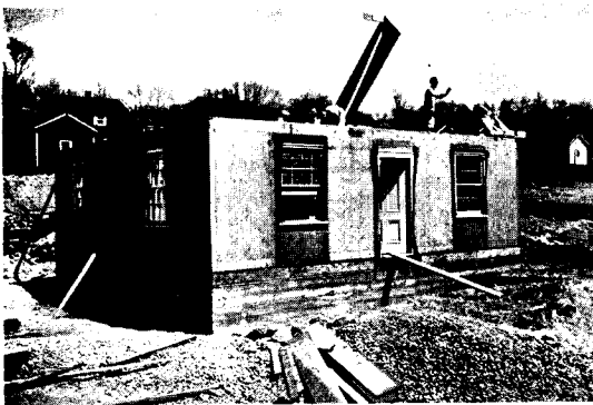
here they demonstrate that a few men can erect the structure in a few hours, in this case starting at 8 A. M., and finishing at 3:55 P. M.
